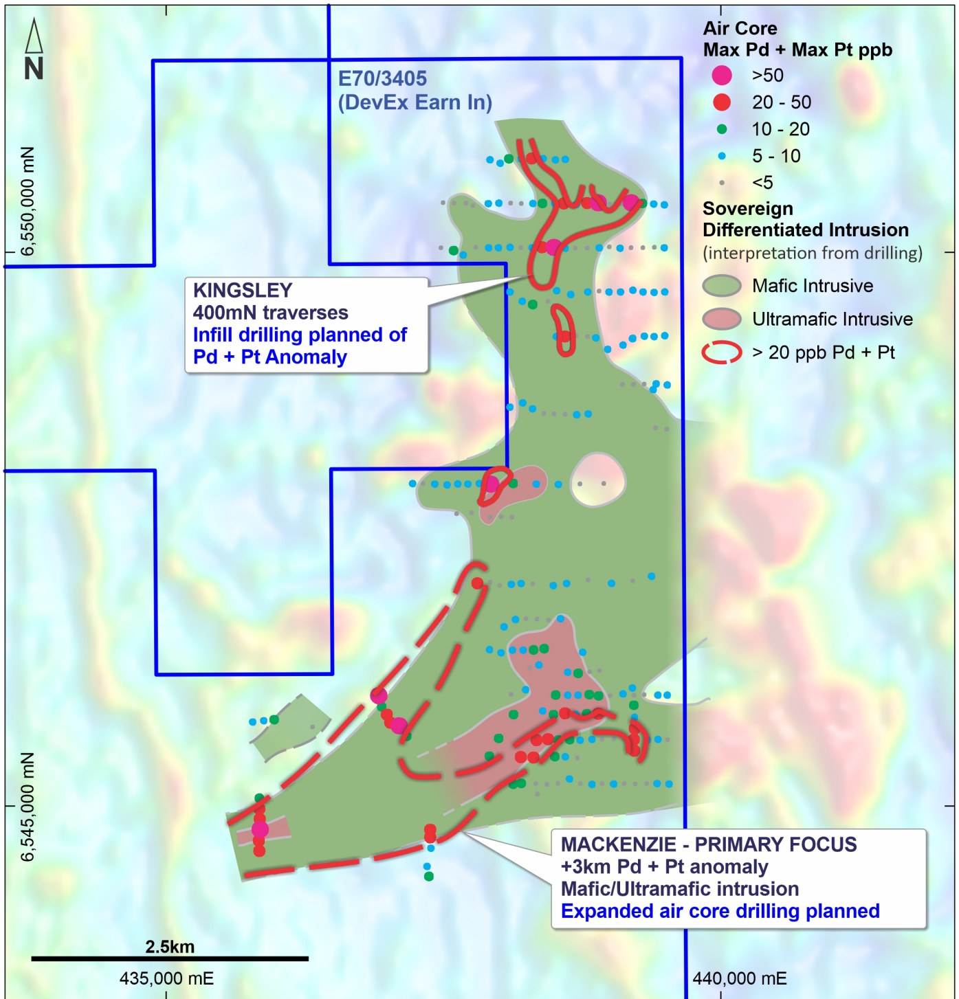
Figure 4: Sovereign Project: DevEx broad spaced air-core drilling and interpreted mafic/ultramafic differentiated intrusion of the Julimar Complex
