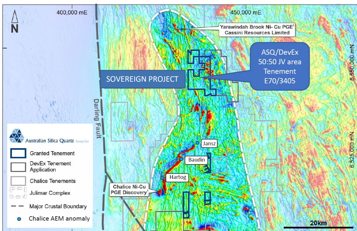
Figure 3: Location of Julimar Complex Sovereign Project with existing Ni-Cu-PGE discoveries on Aeromagnetic RTP image ASQ and DevEx Resources Limited (“DevEx”, ASX: DEV), are engaged in a joint venture, (JV) on the portion of the 6x7km Sovereign magnetic complex located on ASQ’s E70/3405 with DevEx earning-in to the non-bauxite rights of the tenement by an initial spend of $3m to earn a 50% interest with a minimum spend of $250,000. Once DevEx has earned its initial 50% interest, ASQ may elect to contribute to further exploration to maintain its 50% interest, or opt to allow DevEx to spend an additional $3m to earn a further 20% interest with ASQ diluting (ASQ (2020). ASQ Reaches Agreement for Exploration Funding of its Tenement in Julimar Region, WA. ASX Release 1 June 2020).
